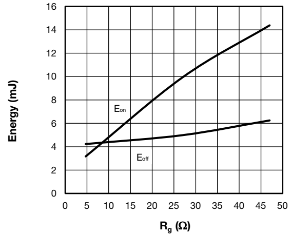
Fig. 9 - Typical Trench IGBT Energy Loss vs. R_g (with Antiparallel Diode) T_J = 125\text{ }^\circ\text{C} , V_{CC} = 600\text{ V} , I_C = 75\text{ A} , V_{GE} = +15\text{V}/-15\text{V} , L = 500\ \mu\text{H}
