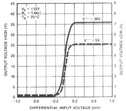
TRANSFER FUNCTION
