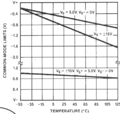
COMMON-MODE LIMITS vs TEMPERATURE
