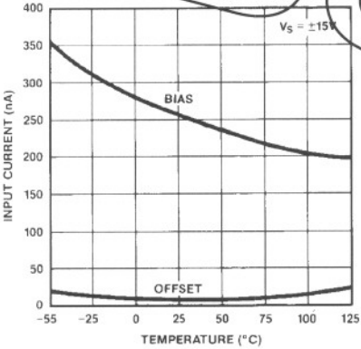
INPUT CURRENTS vs TEMPERATURE
