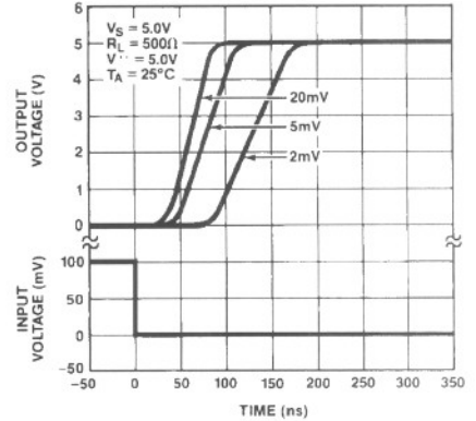
RESPONSE TIMES FOR VARIOUS INPUT OVERDRIVES
