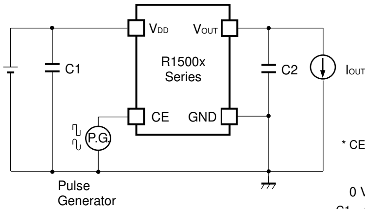
Test Circuit for Turn On Speed with CE pin
