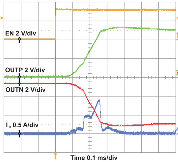
Figure 11. EN Startup
