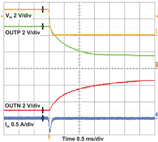
Figure 10. UVLO Shutdown
