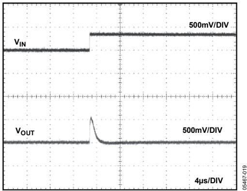
Figure 27. ADR361 Line Transient Response (Increasing), No Capacitors
