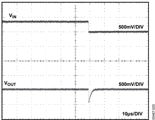
Figure 28. ADR361 Line Transient Response (Decreasing), No Capacitors
