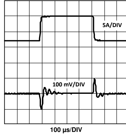
Figure 7-4. V_{IN} = 8\text{ V} , V_{OUT} = 3.3\text{ V} , I_{LOAD} = 11\text{ A} to 19\text{ A} , CH1: V_{OUT} , CH2: I_{LOAD}
