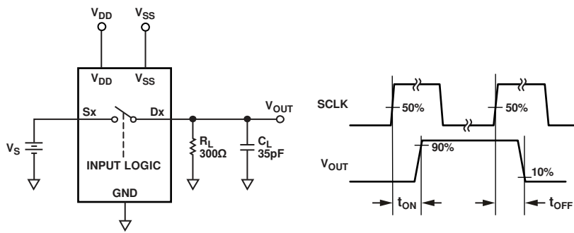
Figure 37. Switching Times, t_{ON} and t_{OFF}
