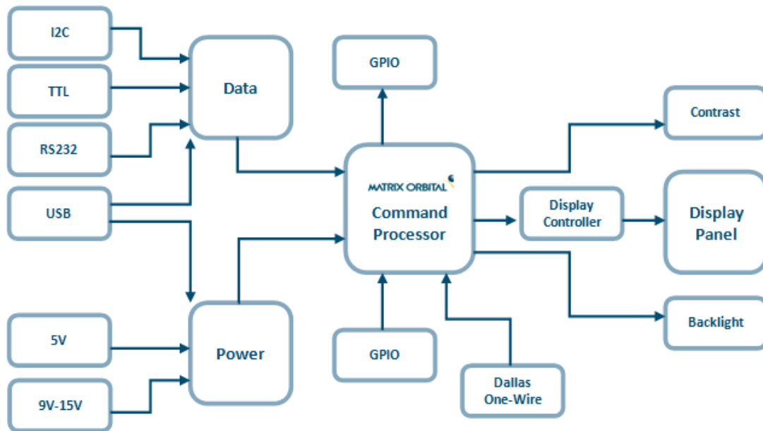
Figure 16: Functional Diagram
