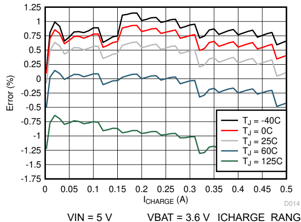
Figure 8-2. Charge Current Accuracy vs. ICHARGE Setting
