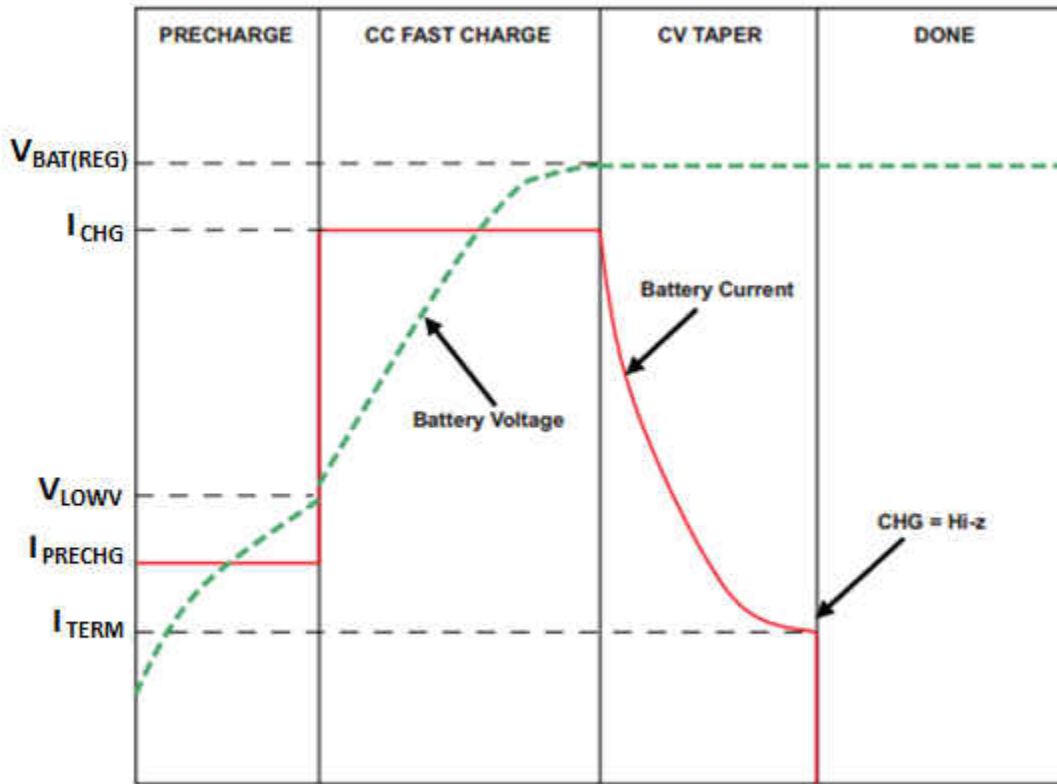
Figure 9-2. BQ25150 Typical Charge Cycle
