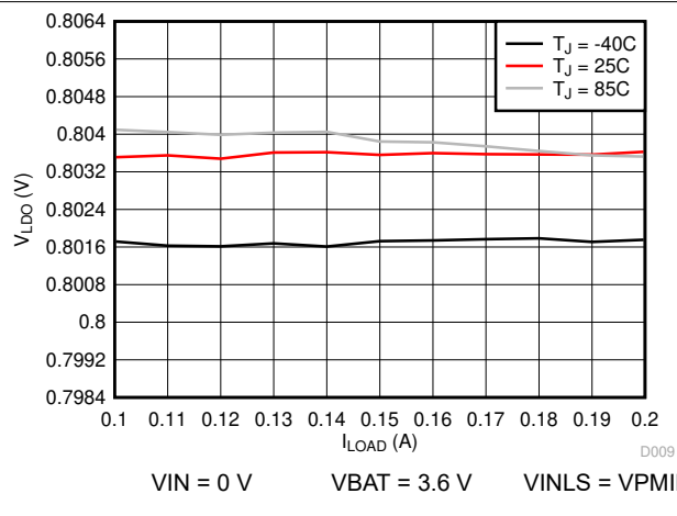
Figure 8-6. LDO Load Regulation (VLDO = 0.8 V)
