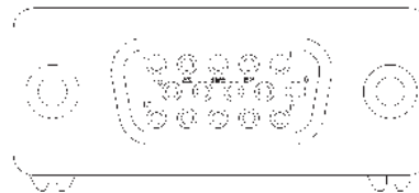
15 Position VESA Receptacle HD-22 Part Number 1734335-1
