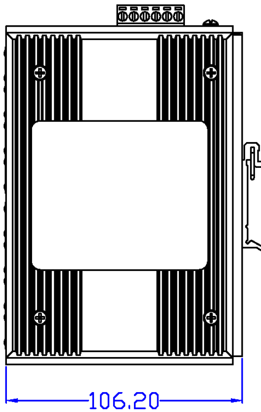
Figure 2.2: Side View of EKI-7526I
