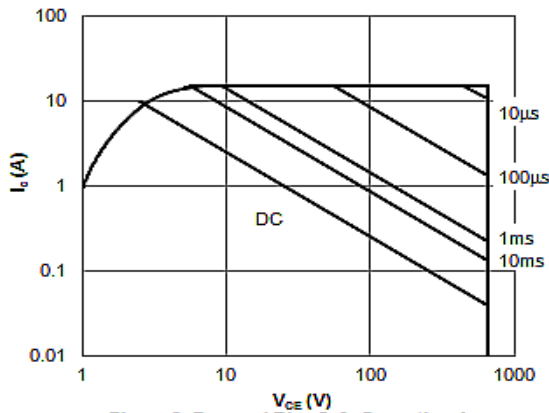
Figure 9: Forward Bias Safe Operating Area ( T_C=25^\circ\text{C} , V_{EE}=15\text{V} )
