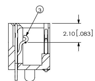
SECTION "A"- "A" SCALE 4 : 1
