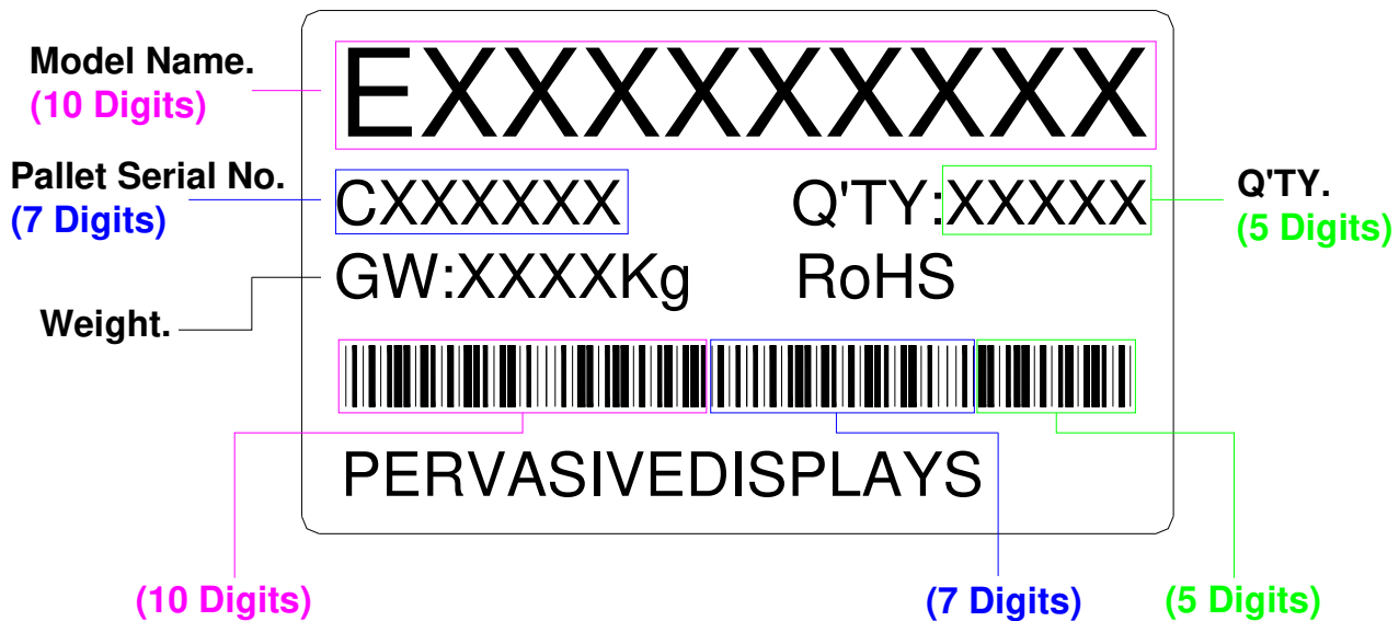
Figure 9-4 Pallet Label
