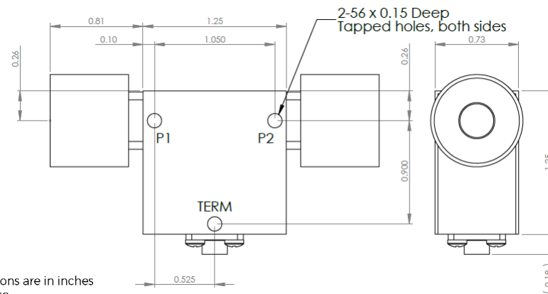
D3I9525N-3 Dimensions
