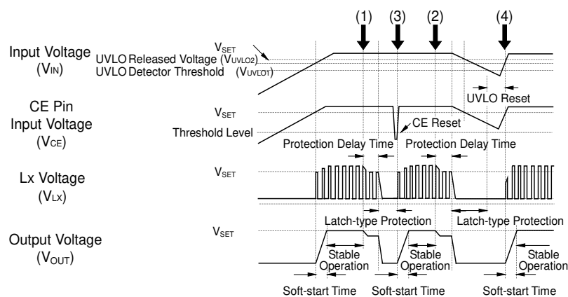
Timing Chart
