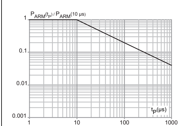
Figure 3. Normalized avalanche power deratings versus pulse duration ( T_j = 125^\circ\text{C} )
