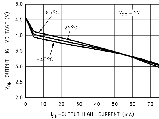
Driver V OH vs I OH vs Temperature
