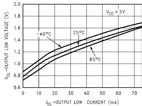
Driver V OL vs I OL vs Temperature
