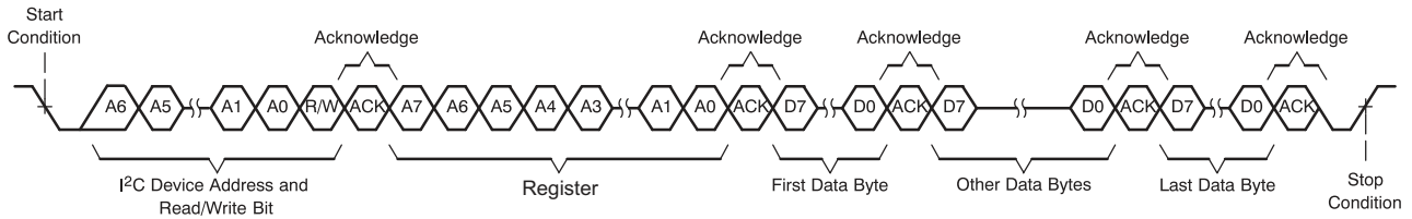
Figure 30. Multi-Byte Write Transfer
