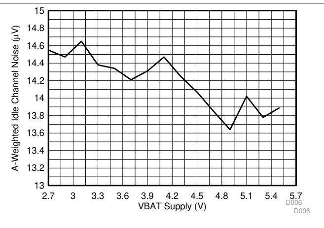
Figure 8. Idle Channel Noise (A-Weighted) vs VBAT
