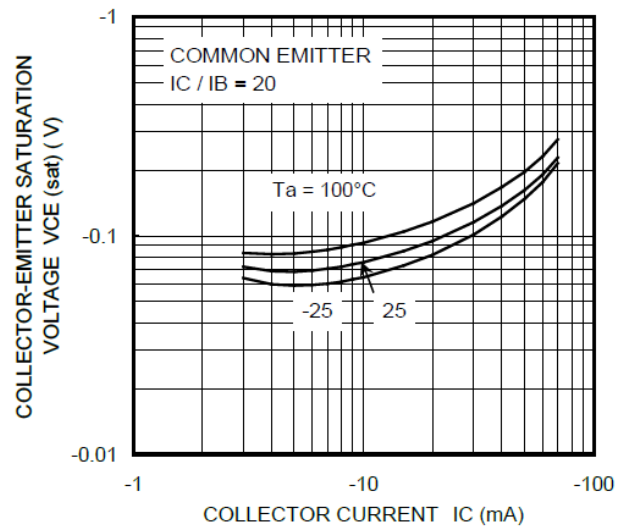
Fig. 10.20 RN2318 V_{CE(sat)}-I_C
