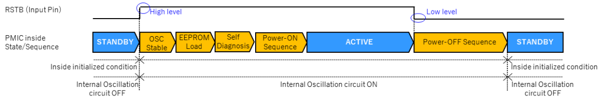
Figure 4. RSTB Operation Timing Chart
