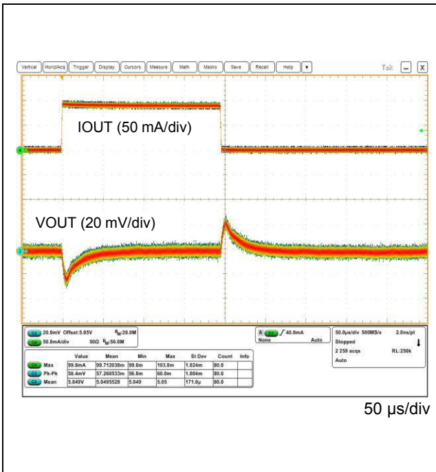
Figure 71. VOUT1 Load Transient (IOUT = 0 A to 100 mA (SR = 100 mA/μs))
