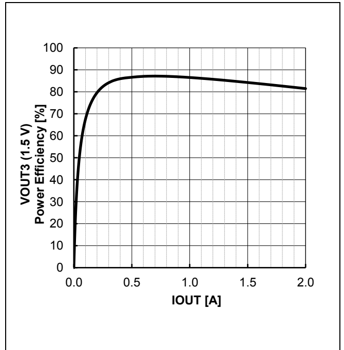
Figure 55. VOUT3 Power Efficiency vs IOU3 (VOUT3 = 1.5 V Setting)
