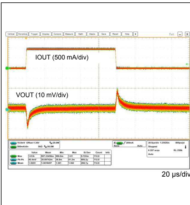
Figure 73. VOUT3 Load Transient (VOUT3 = 1.35 V Setting, IOUT = 0 A to 1 A (SR = 1 A/μs))
