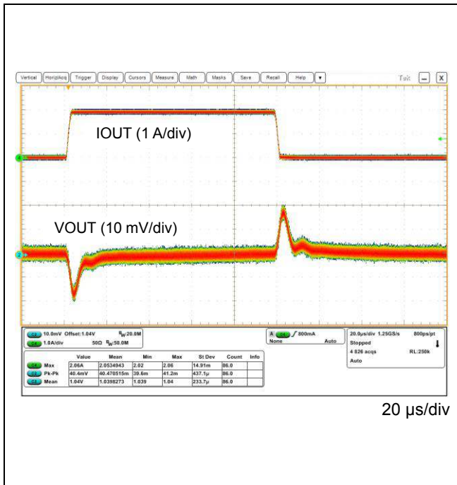
Figure 75. VOUT4 Load Transient (IOUT = 0 A to 2.05 A (SR = 1 A/μs))
