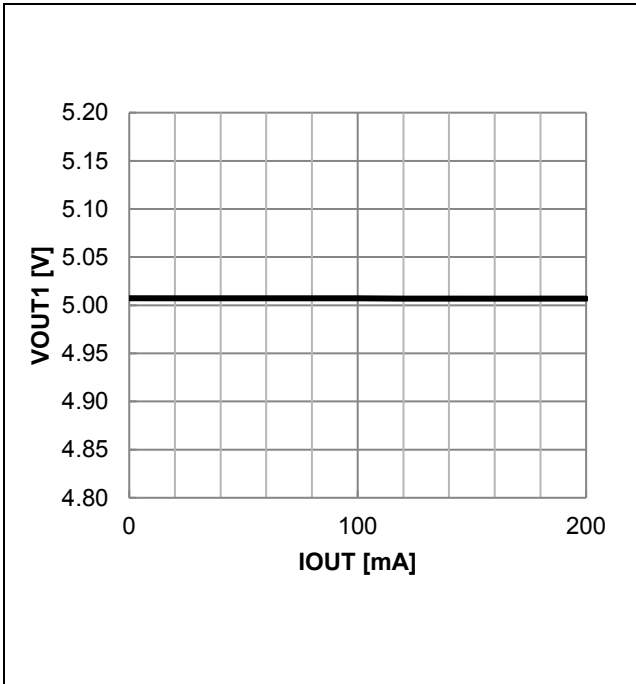
Figure 46. VOUT1 Output Voltage vs IOUT
