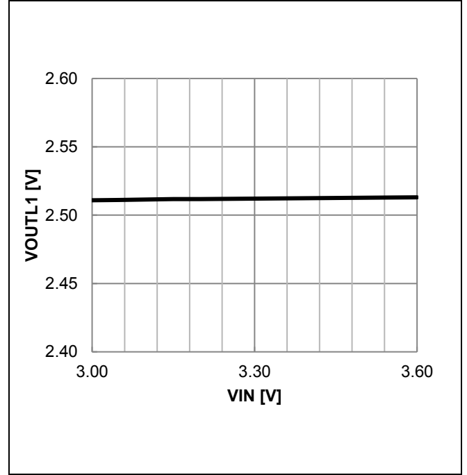
Figure 45. VOUTL1 Output Voltage vs VIN
