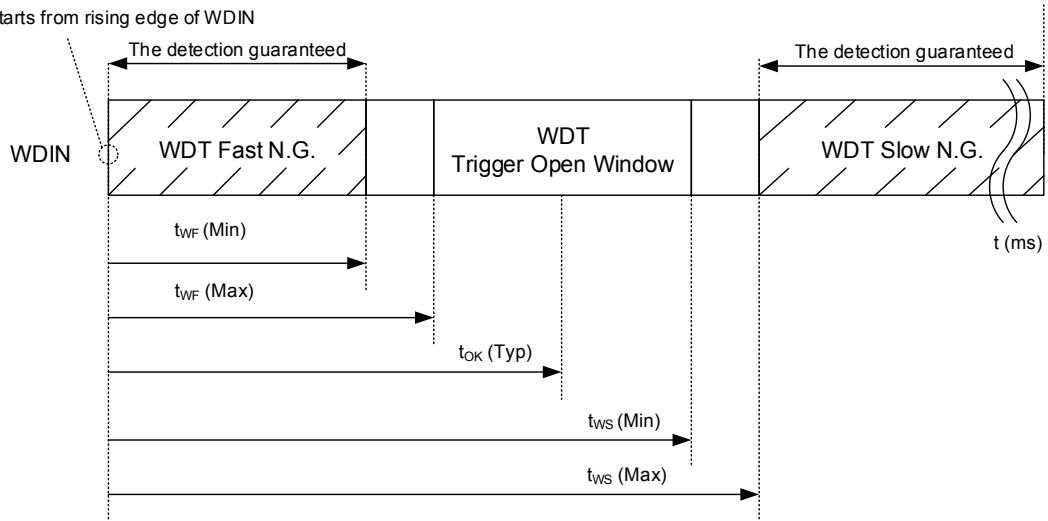
Figure 35. WDT Function
