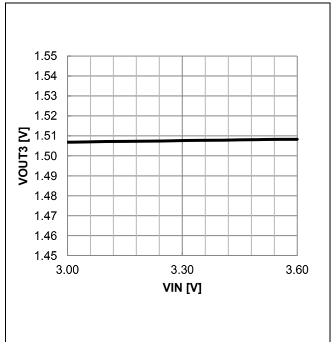
Figure 43. VOUT3 Output Voltage vs VIN (VOUT3 = 1.5 V Setting)
