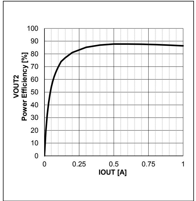
Figure 53. VOUT2 Power Efficiency vs IOU2
