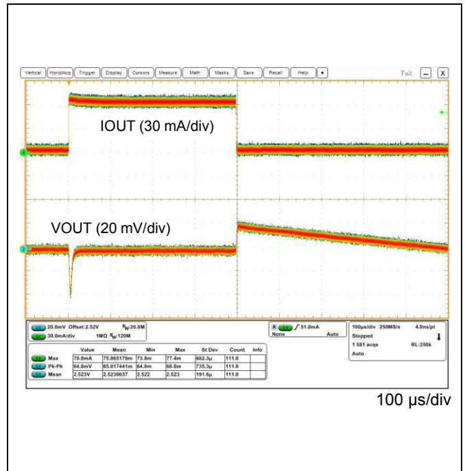
Figure 76. VOUTL1 Load Transient (IOUT = 0 A to 75 mA (SR = 100 mA/μs))
