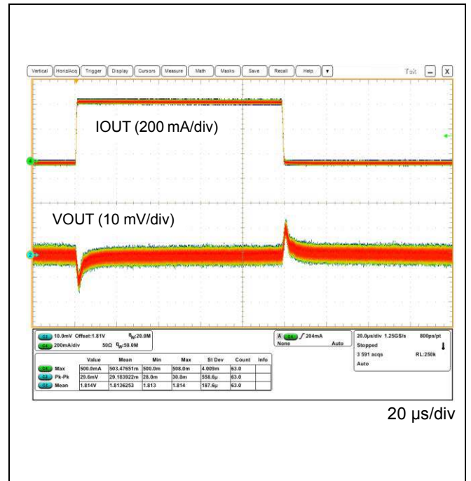
Figure 72. VOUT2 Load Transient (IOUT = 0 A to 0.5 A (SR = 1 A/μs))
