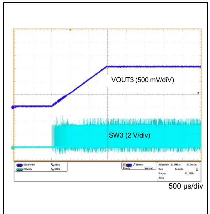
Figure 60. VOUT3 Power ON Waveform (VOUT3 = 1.5 V Setting)
