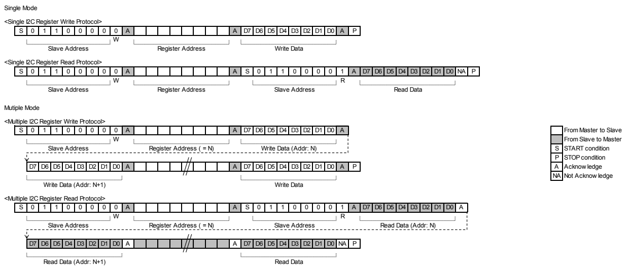
Figure 23. I2C Protocol (Each Access Mode)
