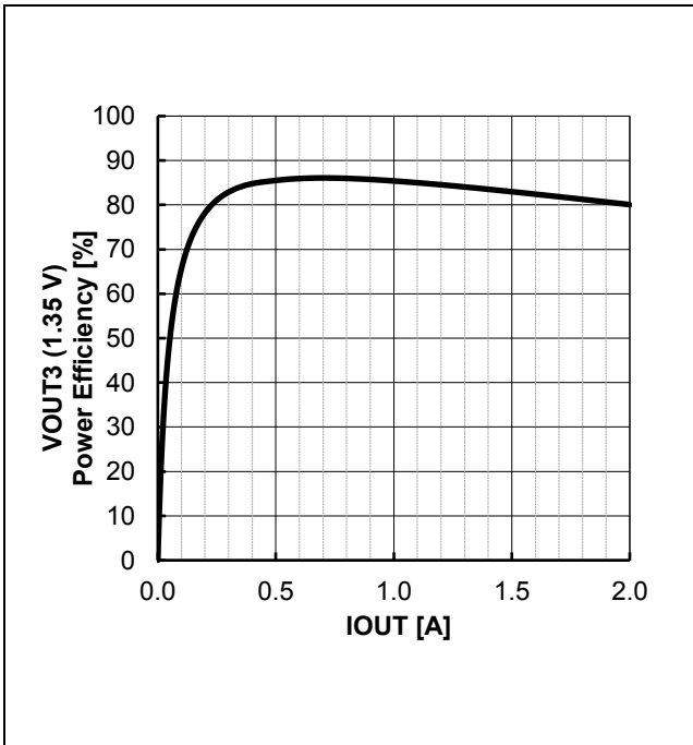
Figure 54. VOUT3 Power Efficiency vs IOU3 (VOUT3 = 1.35 V Setting)
