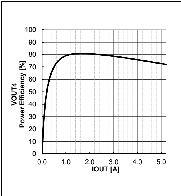
Figure 56. VOUT4 Power Efficiency vs IOUT
