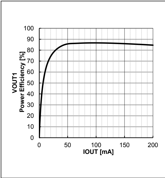
Figure 52. VOUT1 Power Efficiency vs IOU1
