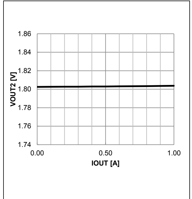
Figure 47. VOUT2 Output Voltage vs IOUT
