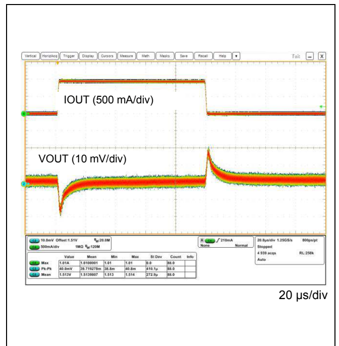
Figure 74. VOUT3 Load Transient (VOUT3 = 1.5 V Setting, IOUT = 0 A to 1 A (SR = 1 A/μs))
