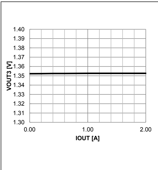
Figure 48. VOUT3 Output Voltage vs IOUT (VOUT3 = 1.35 V Setting)
