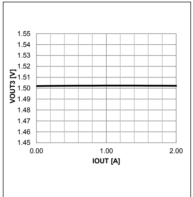
Figure 49. VOUT3 Output Voltage vs IOUT (VOUT3 = 1.5 V Setting)
