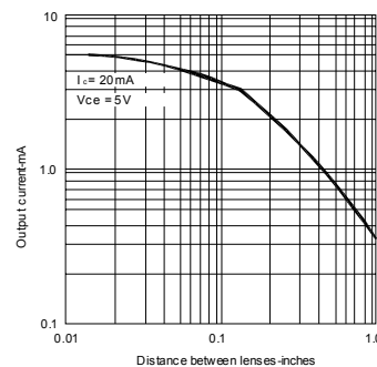
Fig.6 Coupling characteristics
