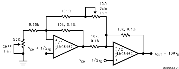
FIGURE 15. Low-Power Two-Op-Amp Instrumentation Amplifier
