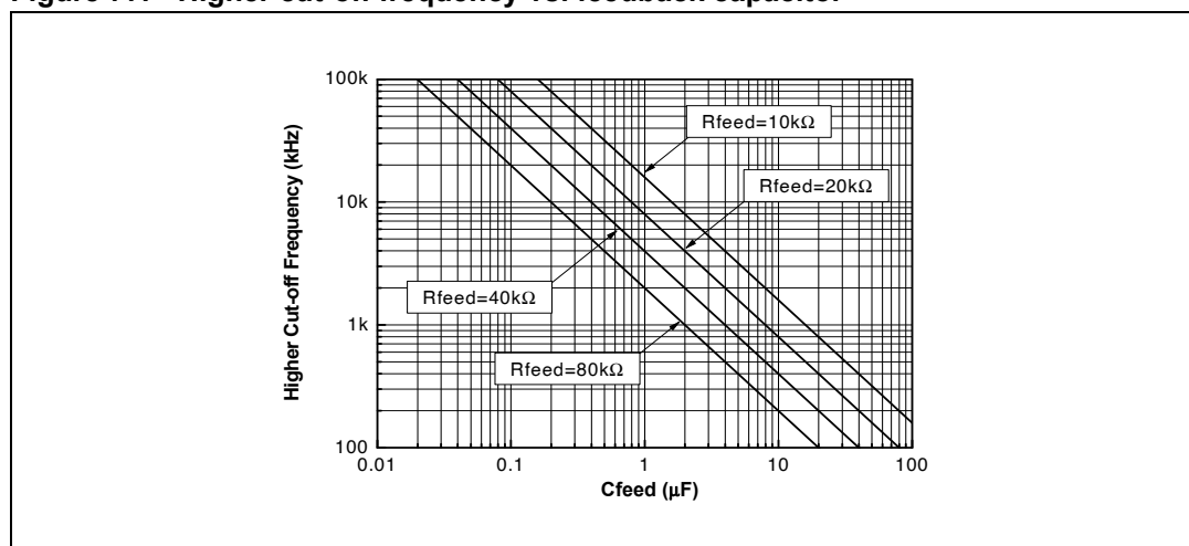
Figure 77. Higher cut-off frequency vs. feedback capacitor
