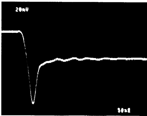
FIGURE 17. DIODE D1 REVERSE RECOVERY WAVEFORM I_F = 200\text{mA} , 20V REVERSE BIAS
