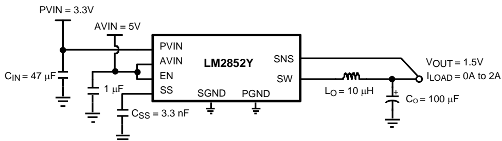
Figure 11. Split-Rail Operation
