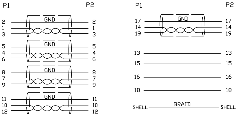
1.Wiring Diagram.
