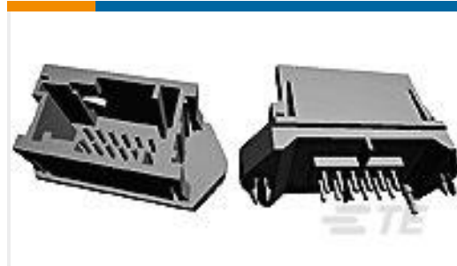
TE Part #953130-3 12pos MQS .63 header 180deg
