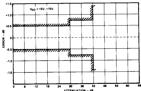
Accuracy Specification for K/B/T Grade Devices at T_A = +25^\circ C
