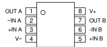
MSOP-8
