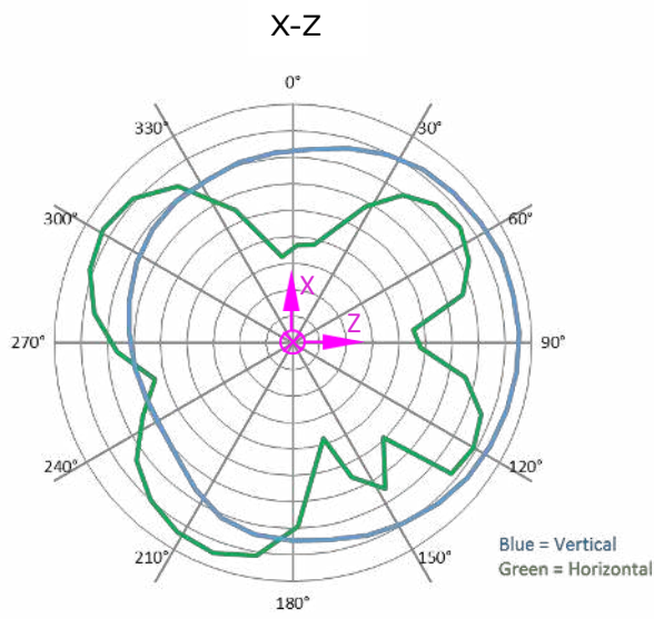
Figure 11: X-Z plane antenna pattern
