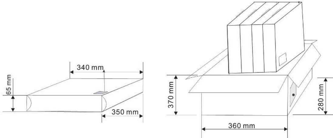
Figure 13: Reel cartons used for type number BMD-300-A-R-00
