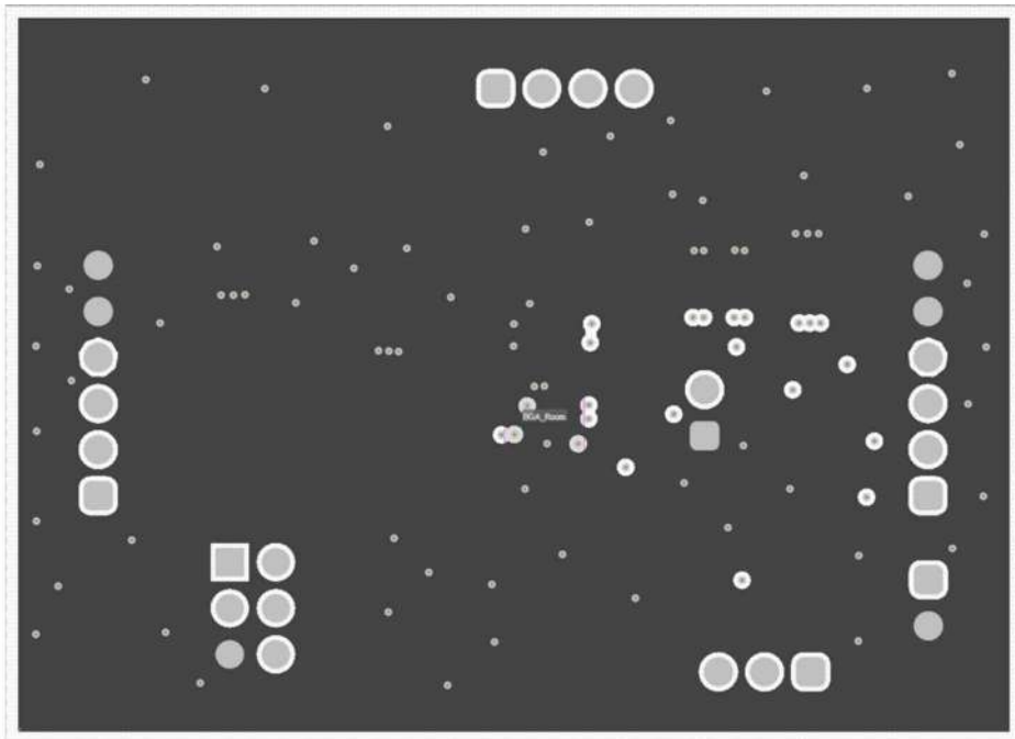
Figure 6-3. Internal Layer 1
