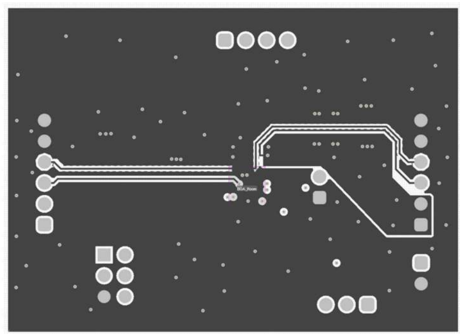
Figure 6-4. Internal Layer 2
