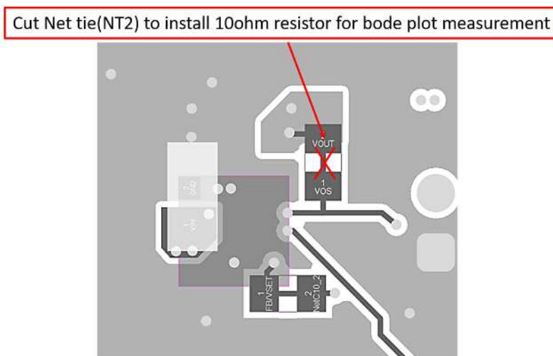
Figure 3-2. Bode Plot Measurement Board Modification
