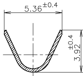
SECT. B-B
