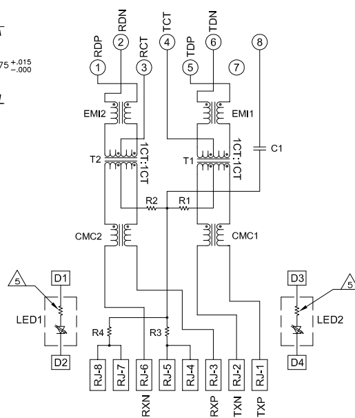
706 10/100 BASE-T CIRCUIT
