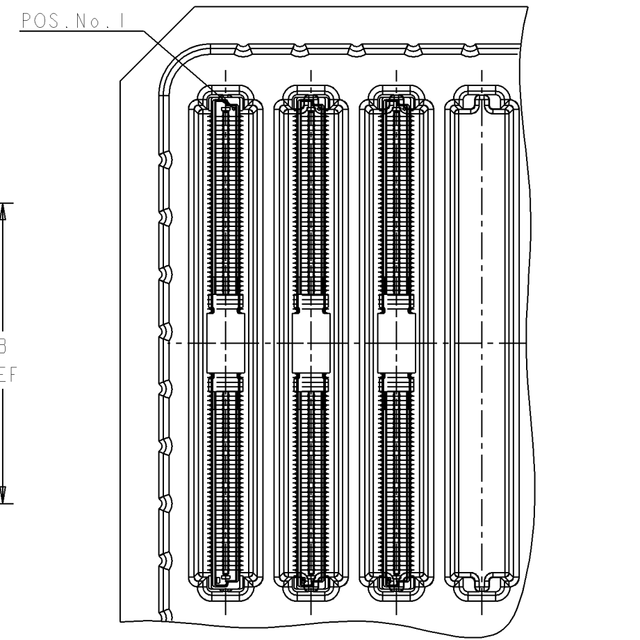
DETAIL "A" (1X EMPTY POCKET SHOWN FOR REF.)
