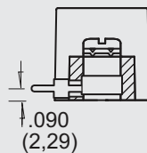
CBDR right angle printed circuit disconnect
