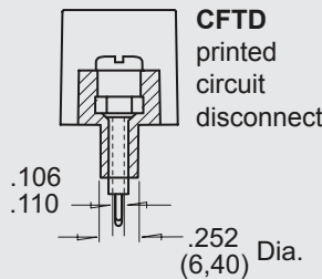
CFTD printed circuit disconnect CFTD is normally supplied with standard pin installed.
