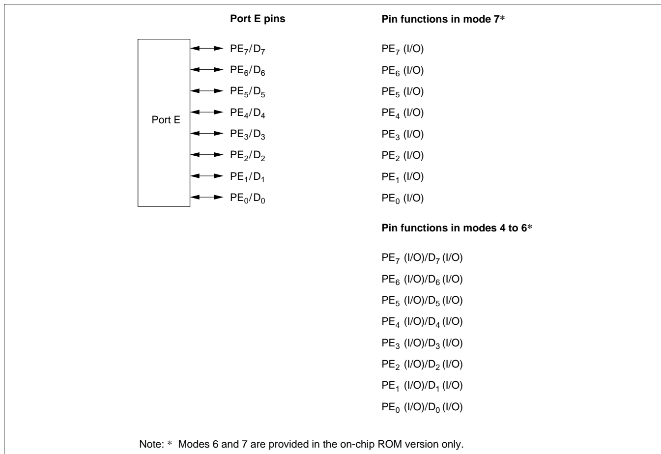
Figure 9-22 Port E Pin Functions
