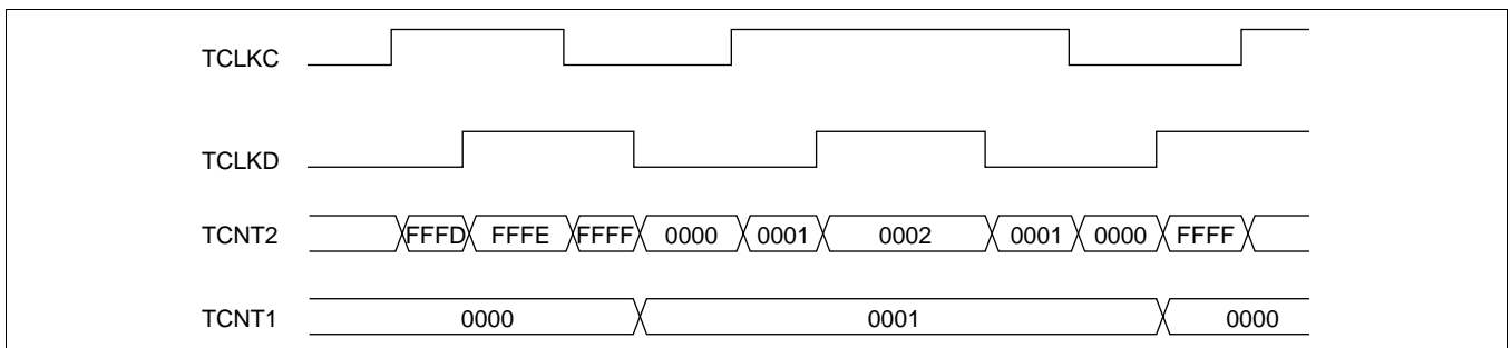
Figure 10-23 Example of Cascaded Operation (2)
