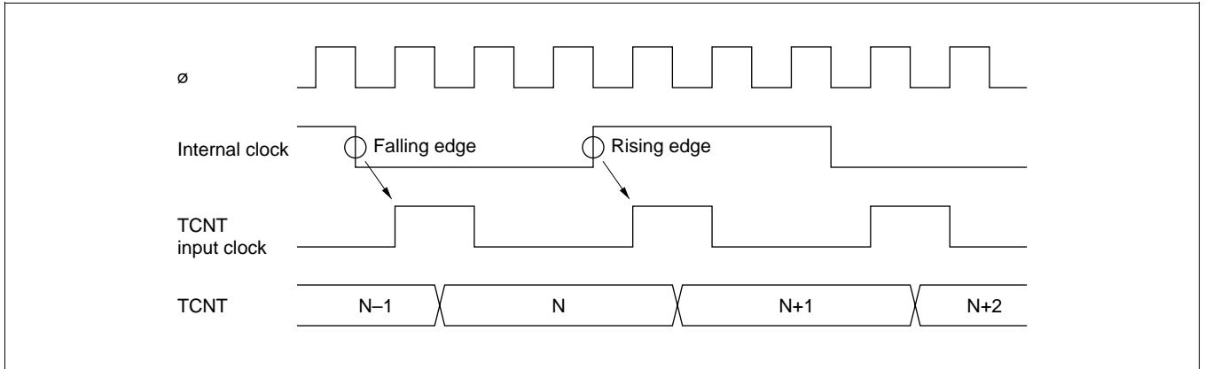
Figure 10-34 Count Timing in Internal Clock Operation
