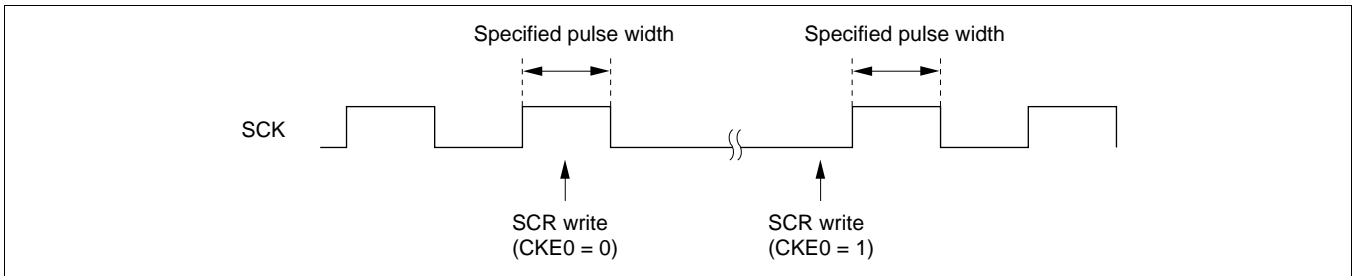
Figure 15-8 Timing for Fixing Clock Output Level
