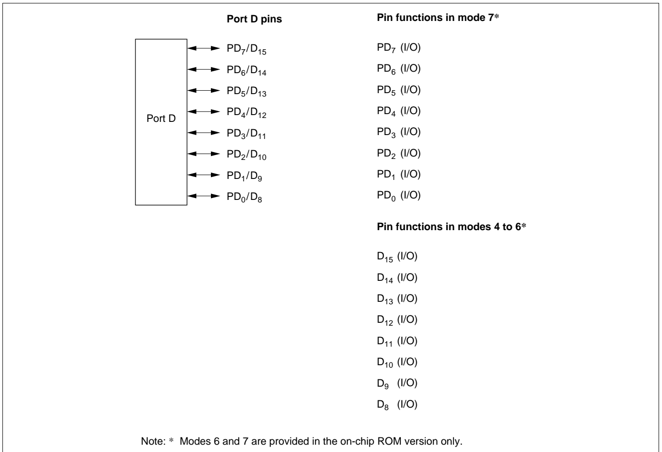
Figure 9-19 Port D Pin Functions
