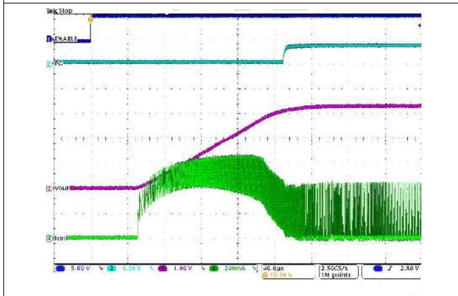
Iout = 100 mA
