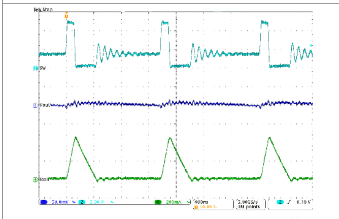
Iout = 66 mA
