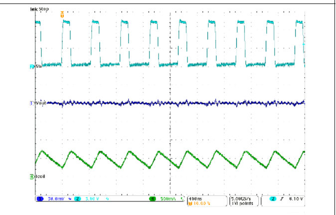
Iout = 500 mA
