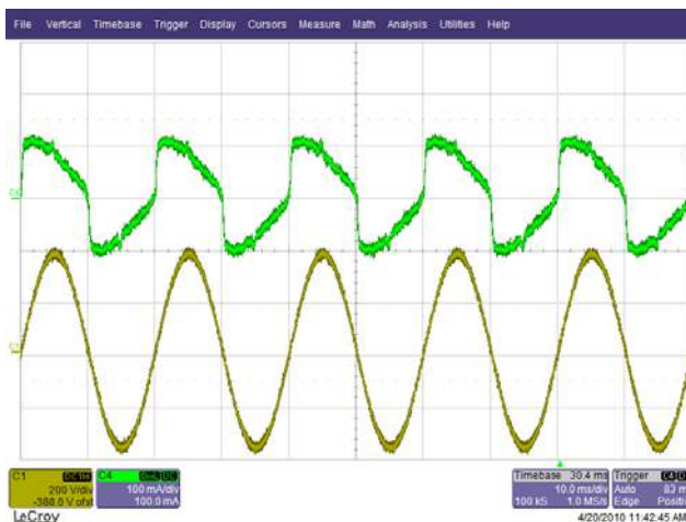
Figure 18 – 265 VAC, Full Load. Upper: I_{IN} , 0.1 A / div. Lower: V_{IN} , 200 V / div., 10 ms / div.
