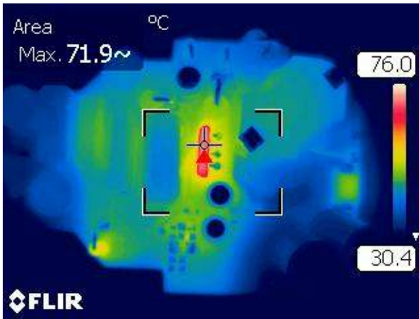
Figure 11 – Top Side.
