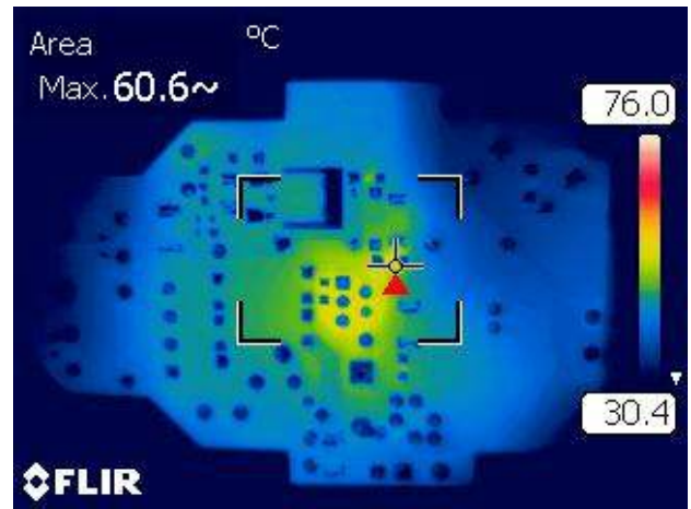
Figure 12 – Bottom Side.
