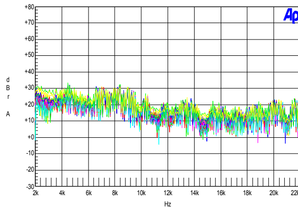
Figure 44 – 2 kHz – 22 kHz.
