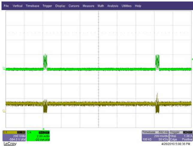
Figure 25 – 90 VAC, Full Load. Upper: I_{OUTPUT} , 2 A / div. Lower: V_{DRAIN} , 200 V, 200 ns / div.
