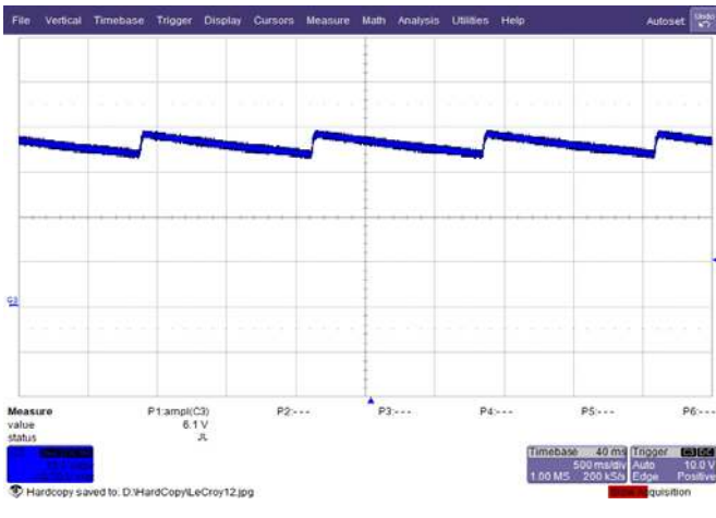
Figure 27 – Output Voltage: 115 VAC. V_{OUT} , 10 V / div., 500 ns / div.
