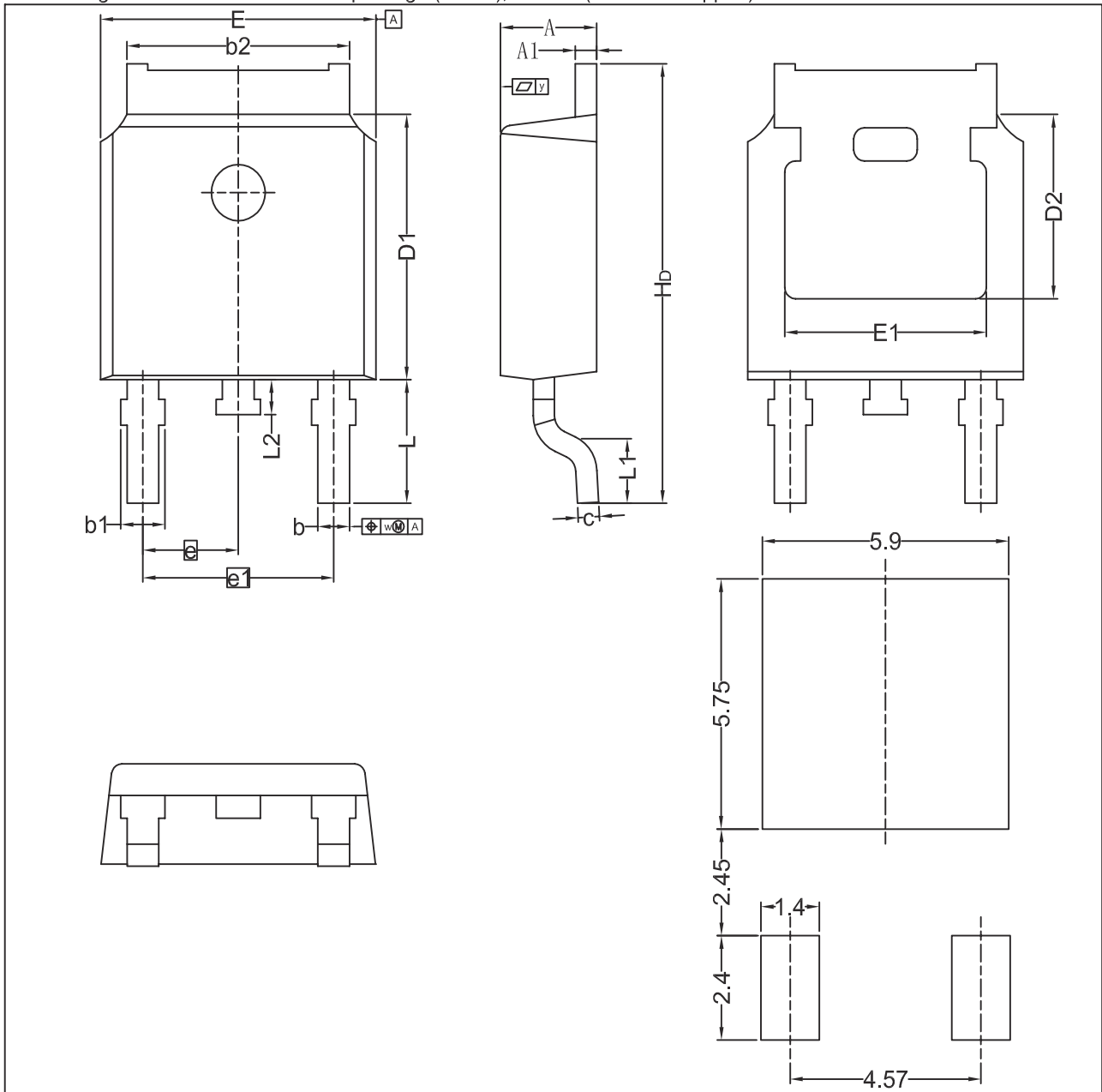
Recommended Footprint
