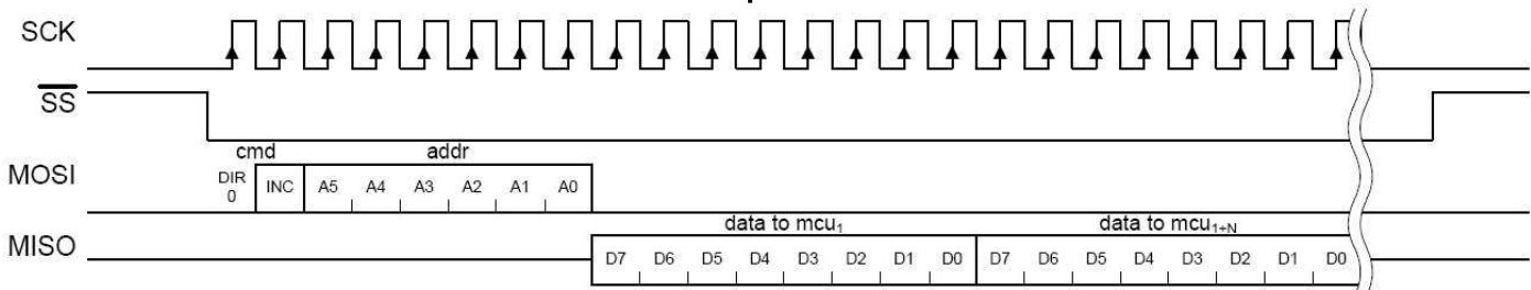
Figure 4 - SPI Incrementing Burst Read Sequence
