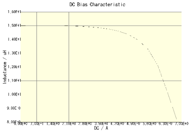
CLF12555T-150M-CA(Amb. Temp. = 20degc)
