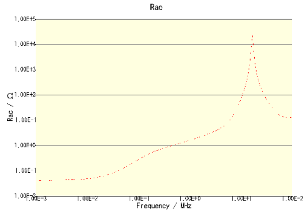
CLF12555T-150M-CA
