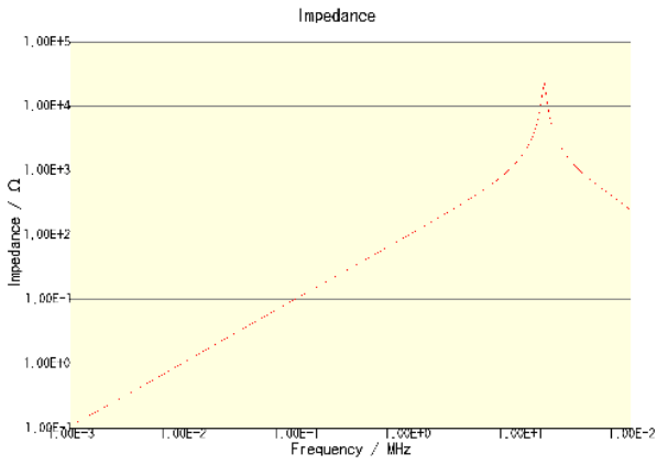
CLF12555T-150M-CA
