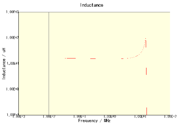
CLF12555T-150M-CA
