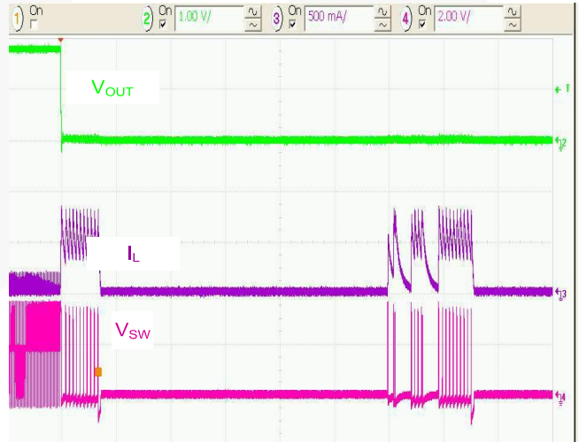
Figure 16. Metallic Short Applied at V OUT , 50μs/div.
