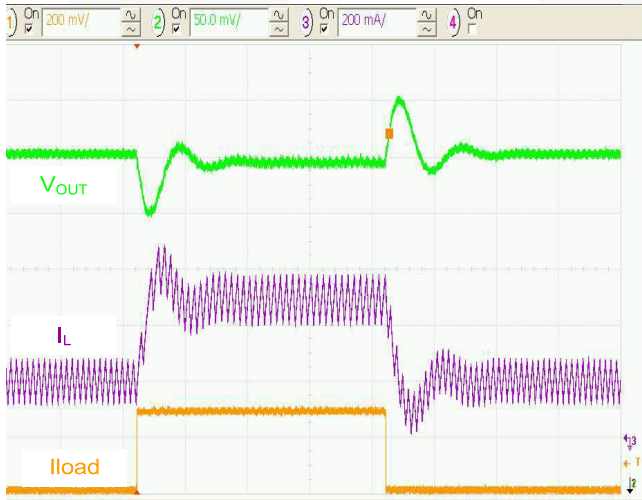
Figure 15. Load Transient 200 to 500mA, 3.6V IN , 5μs/div.
