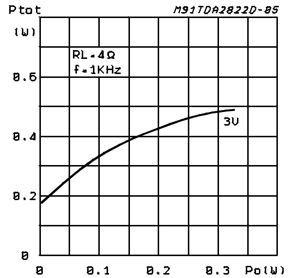
Figure 8. Total power dissipation vs. output power (bridge, RL=4 Ω)
