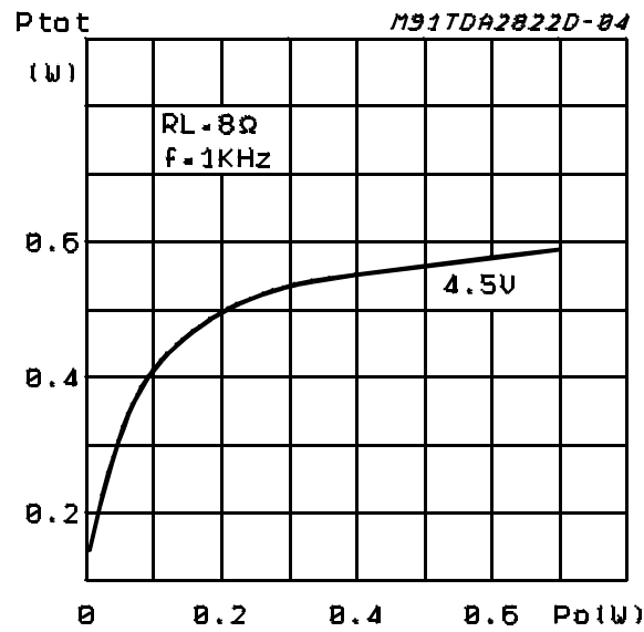
Figure 7. Total power dissipation vs. output power (bridge, RL=8 Ω)
