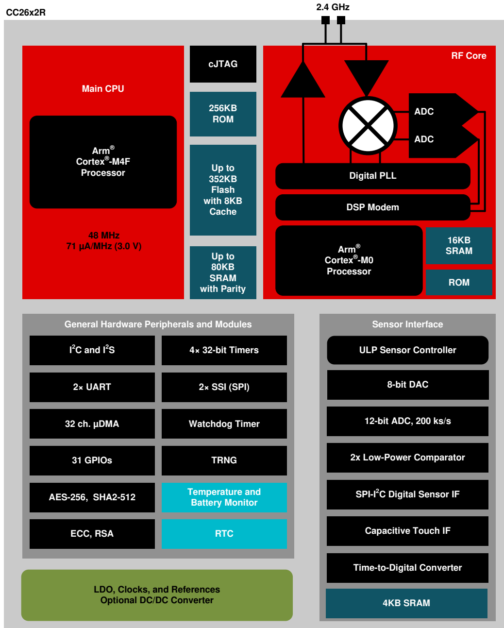
Figure 4-1. CC2642R Block Diagram
