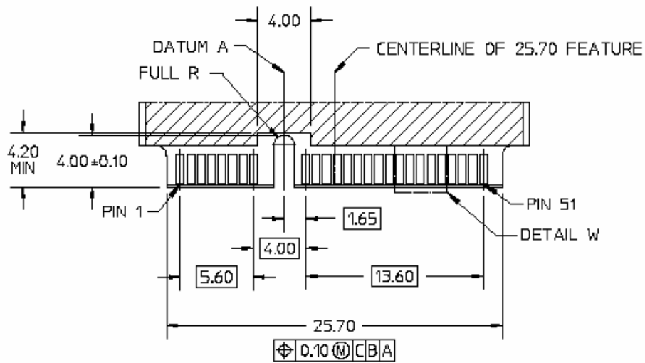
DETAIL Z
