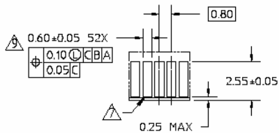
DETAIL W
