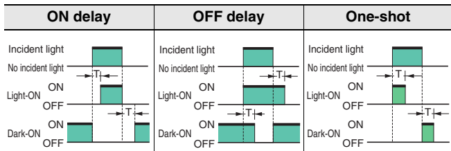
Note: Timing Charts for Timer Settings (T: Set Time)
