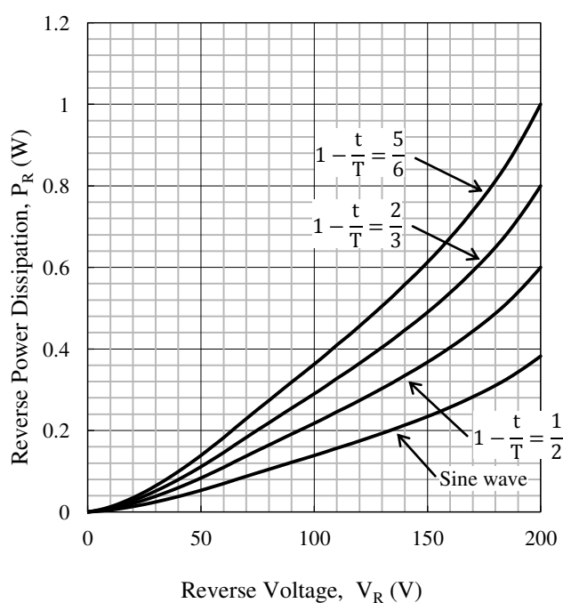
Figure 3-11 P_R - V_R
