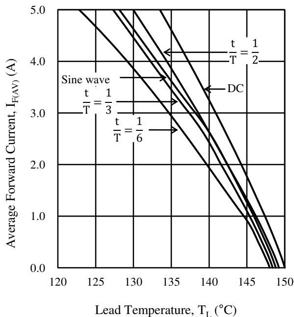
Figure 3-7 I_{F(AV)} - T_L ( V_R = 200\text{ V} )
