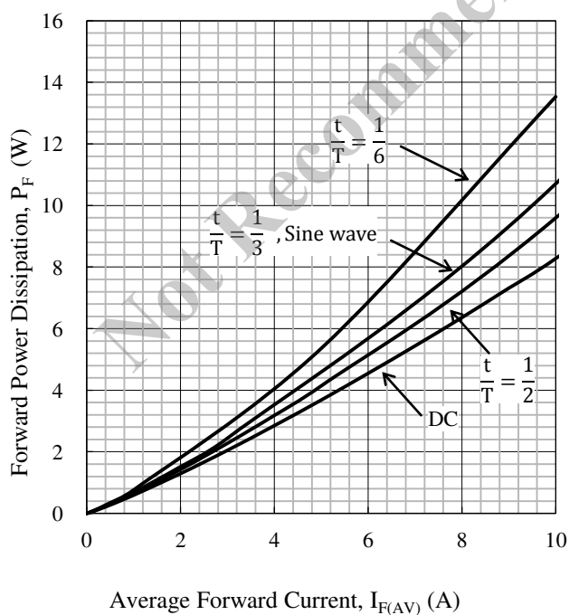
Figure 3-10 P_F - I_{F(AV)}
