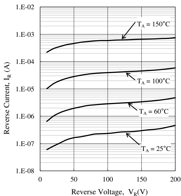
Figure 3-15 V_R - I_R Typical Characteristics
