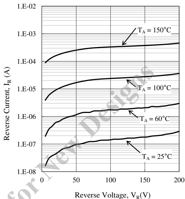
Figure 3-9 V_R - I_R Typical Characteristics
