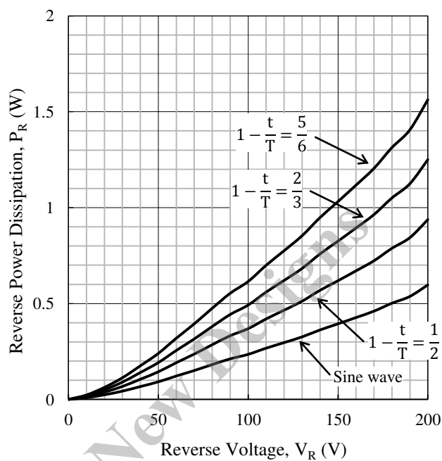
Figure 3-17 P_R - V_R
