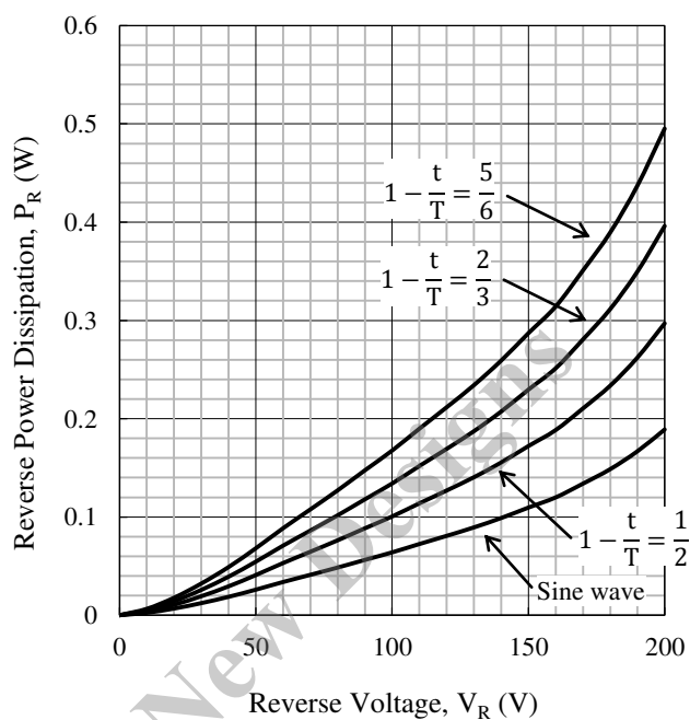
Figure 3-5 P_R - V_R
