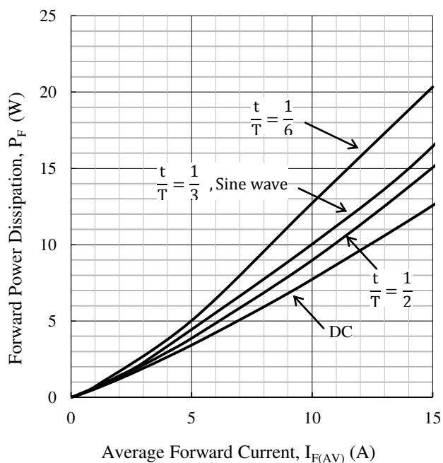
Figure 3-16 P_F - I_{F(AV)}
