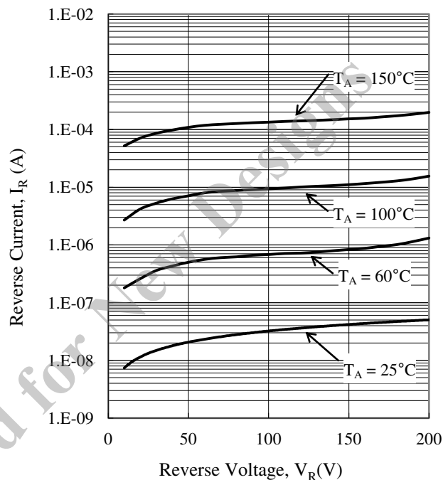
Figure 3-3 I_R - V_R Typical Characteristics
