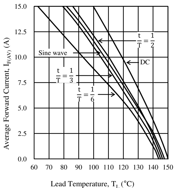
Figure 3-19 I_{F(AV)} - T_L ( V_R = 200\text{ V} )
