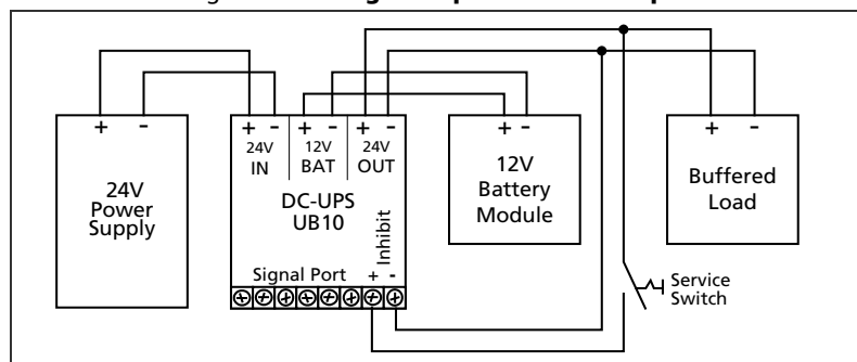
Fig. 26-3 Wiring example for inhibit input
