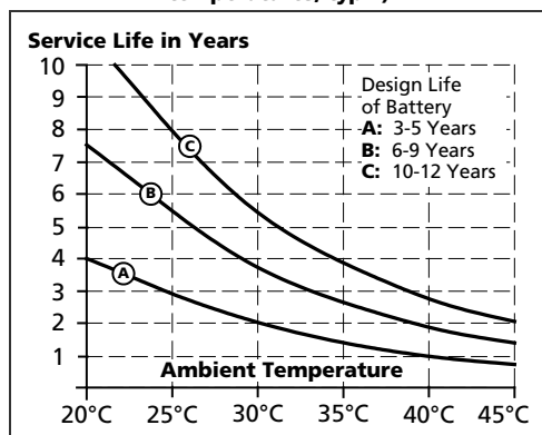
Fig. 26-1 Service life versus ambient temperatures, typ *)
