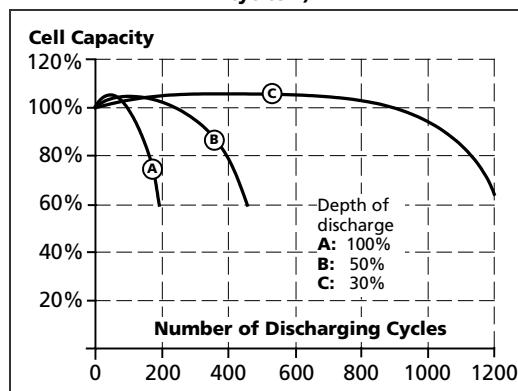
Fig. 26-2 Cell capacity degradation vs. discharging cycles *)
