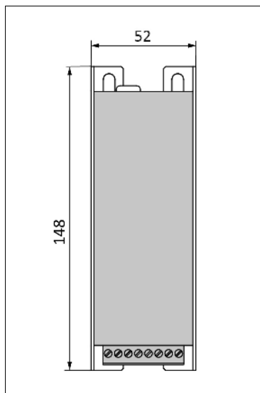
Fig. 25-5 Wall/panel mounting, side view
