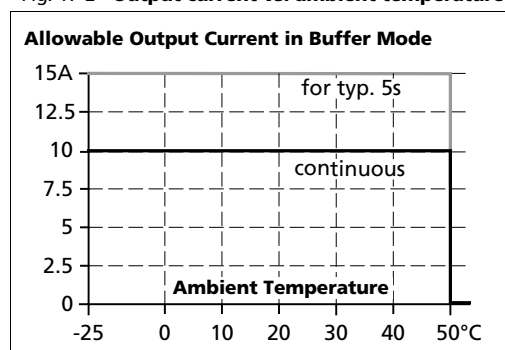
Fig. 17-2 Output current vs. ambient temperature
