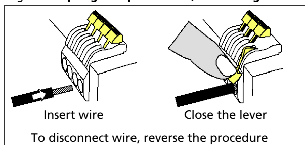
Fig. 14-1 Spring-clamp terminals, connecting a wire
