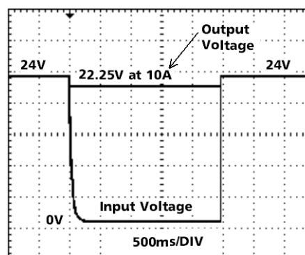
Fig. 5-2 Transfer behavior, typ.
