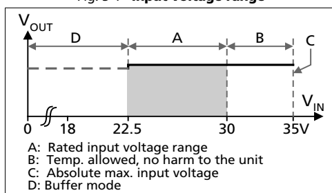
Fig. 3-1 Input voltage range
