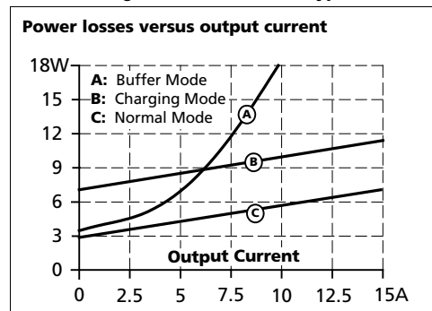
Fig. 8-2 Losses at 24V, typ.
