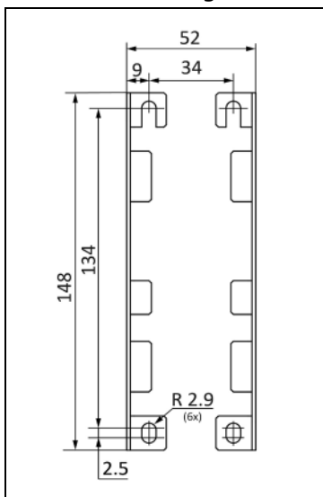
Fig. 25-6 Hole pattern for wall mounting
