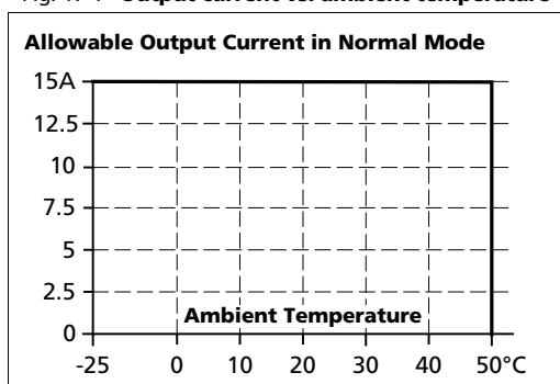
Fig. 17-1 Output current vs. ambient temperature
