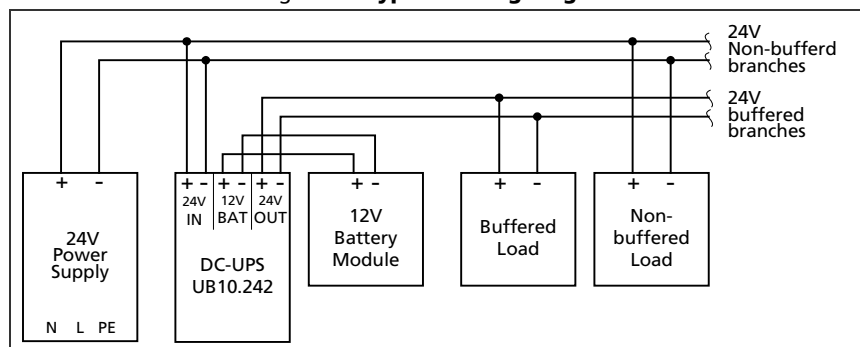
Fig. 24-1 Typical wiring diagram
