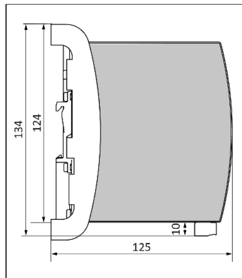
Fig. 25-7 Wall/panel mounting, side view
