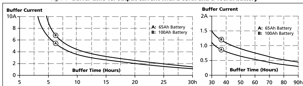
Fig. 7-1 Buffer time vs. output current with a 65Ah and a 100Ah battery
