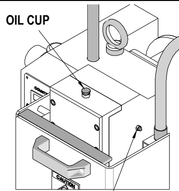
Figure 4-8 GREASE FITTING
